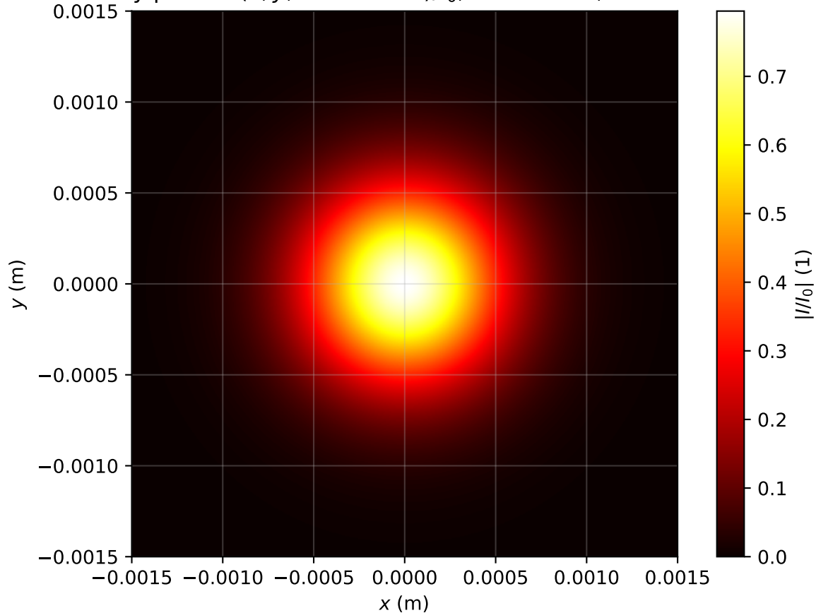
Intensity profile I(x, y, z = 1.513m)/I_0 , \text{Pin}=0.3\text{Pcr} , artificial time
